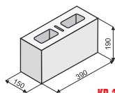
KB 1-15 A
