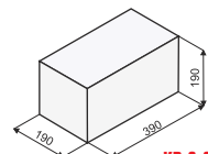
KB 2-20 A
