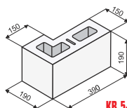
KB 5-15 A
