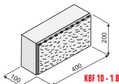
KBF 10 - 1 B
