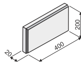
KBF 0-11 A 20
