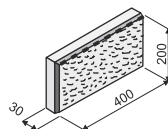
KBF 0-11 B 30
