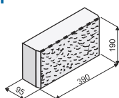
KB 2-11 B 390
