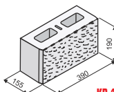
KB 1-15 B
