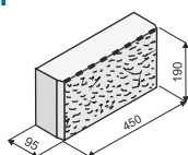
KB 2-11 B 450
